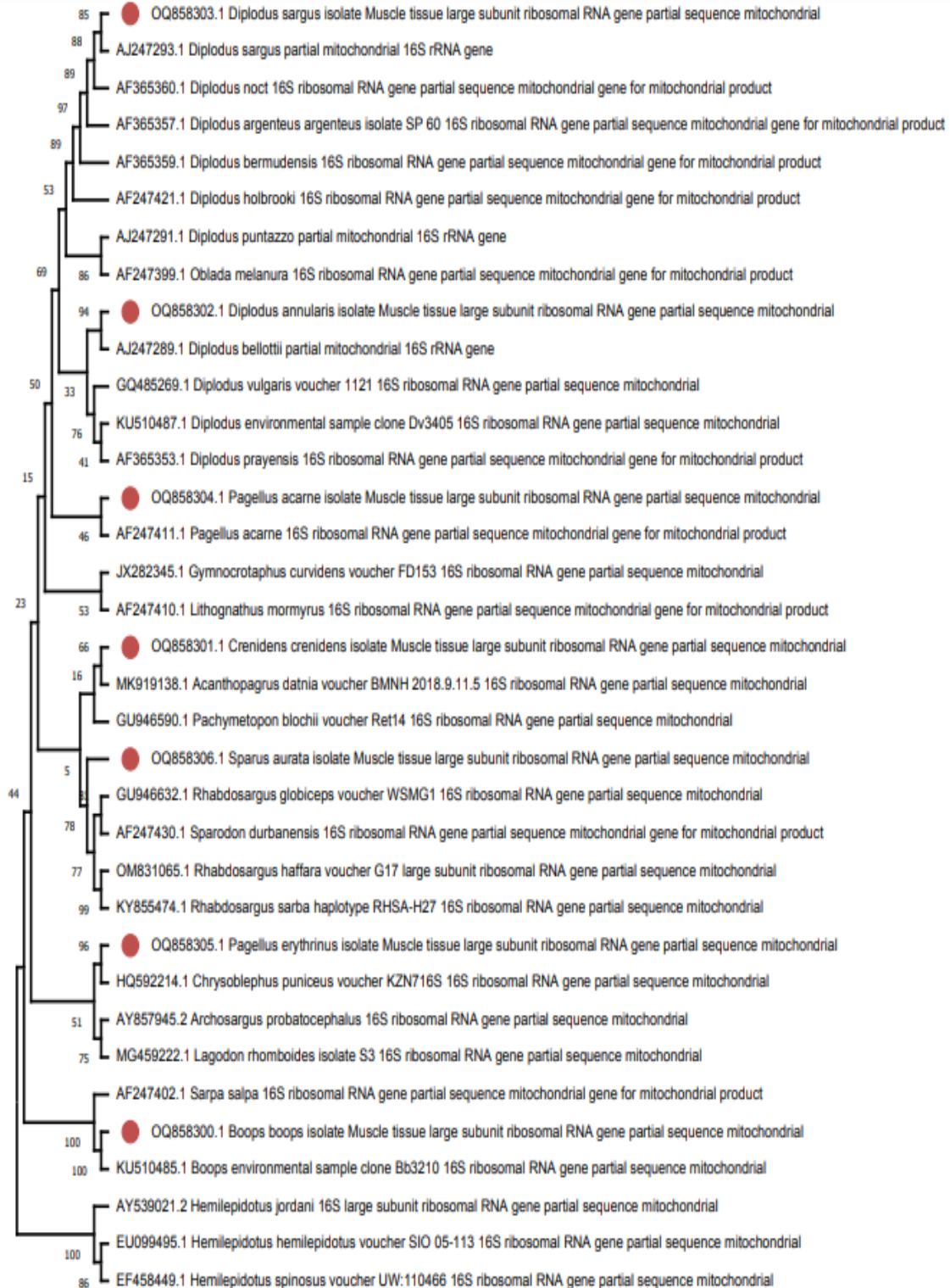
Fig. 3. Minimum evolution phylogenetic tree in seven sparid fish and their linked sparid species with the outgroup by employing the 16S rRNA gene
